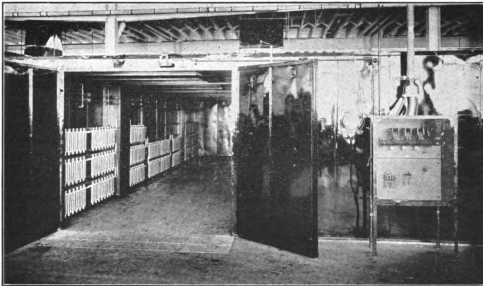
Interior of half of automobile body baking oven with General Electric Co. heaters and automatic control panels. Oven 40 x 20 ft.; 441 k.w.
